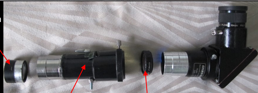
Adjustable Fabry-Perot etalon filter compartment
