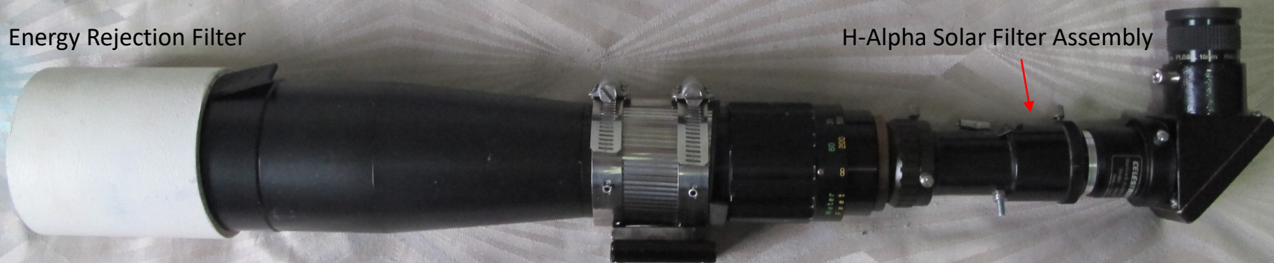
Old 400mm Film Camera Telephoto Lens
